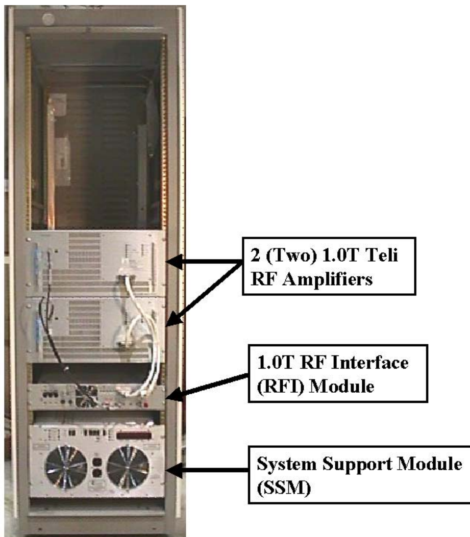
1.0T SRF CABINET ILLUSTRATION 1-1
