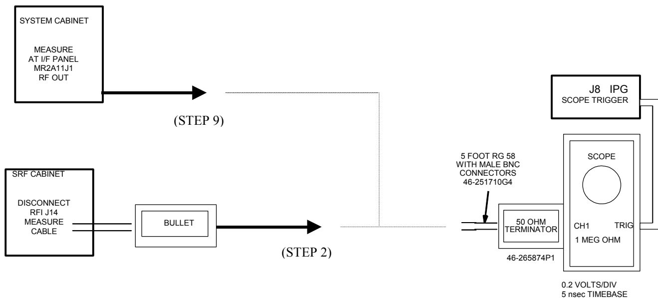
RF SIGNAL MEASUREMENTS USING A SCOPE OF \geq 100 MHZ BANDWIDTH ILLUSTRATION D1-1
